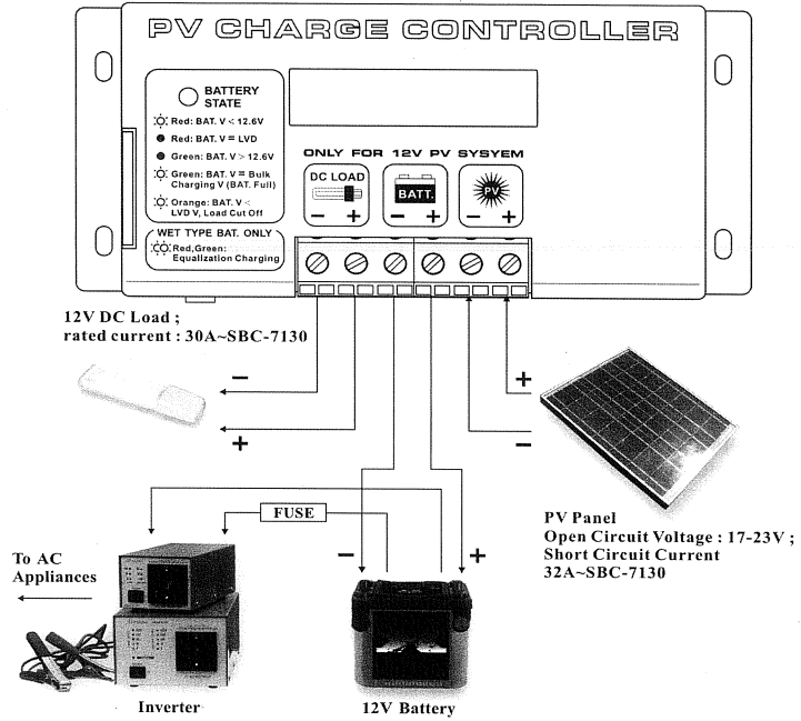
Figure 2 Connection of PV Charge Controller
