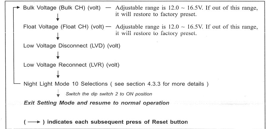
Figure 6 Adjustable parameters in Setting Mode
