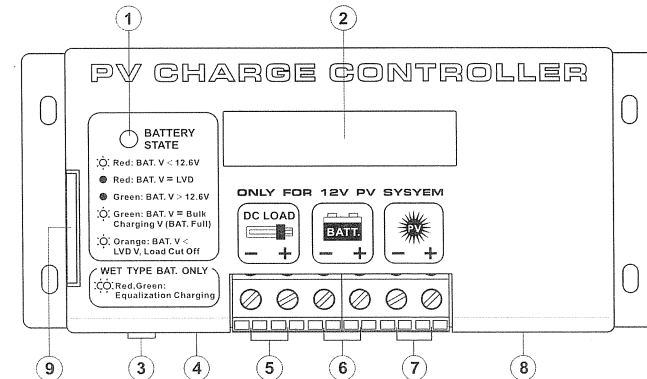
Figure 1 Front view of PV Charge Controller
