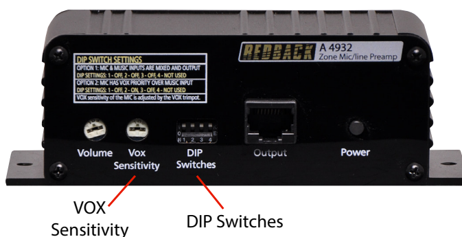
Fig 5 - A 4932 DIP switches and VOX sensitivity adjustment location.
