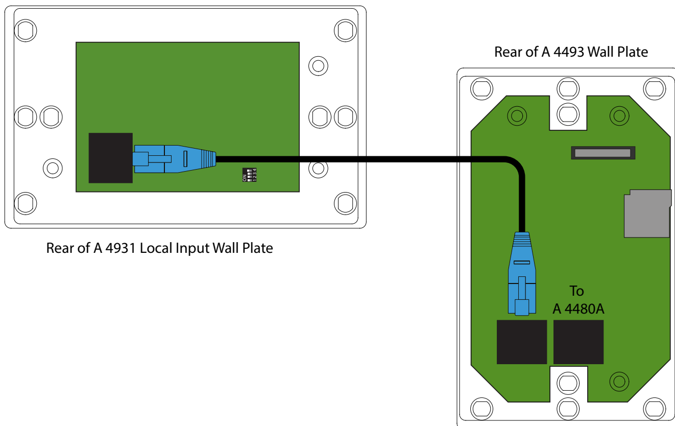
Fig 5.6 Connection of the A 4931 Local Input Wall Plate to the A 4493 Input Source Wall Plate
