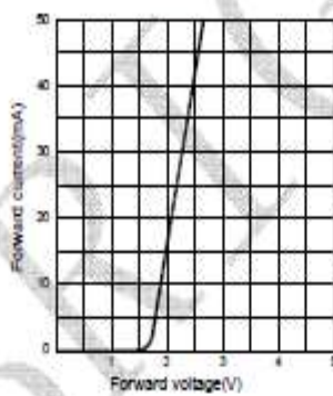
Fig.3 Forward current vs. Forward voltage
