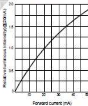
Fig.5 Relative luminous Intensity vs. Forward current
