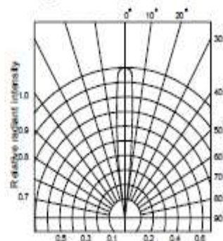
Fig.6 Radiation diagram
