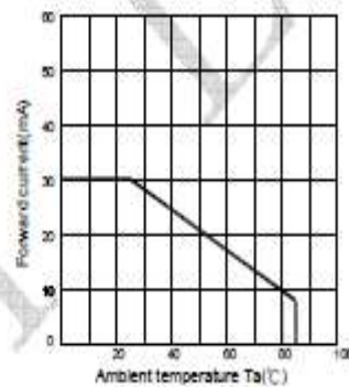
Fig.2 Forward current derating curve vs. Ambient temperature
