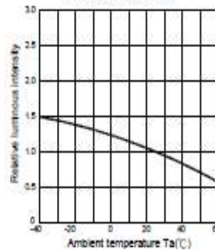
Fig.4 Relative luminous intensity vs. Ambient temperature
