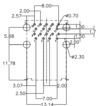
P. C. Board Layout
