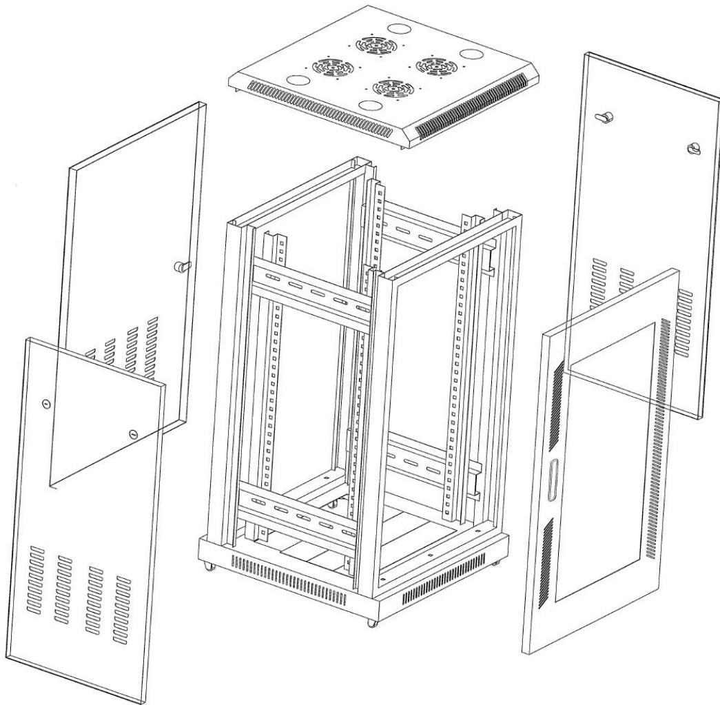
Sample Rack System – Exploded Panels View
