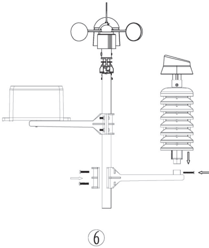
Mounting the thermo-hygro sensor same as rain sensor
