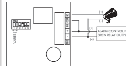
Fig. 6 – Pulse/flash o/p, instant/delay
