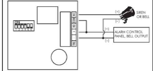
Fig. 5 – Latched output, delayed
