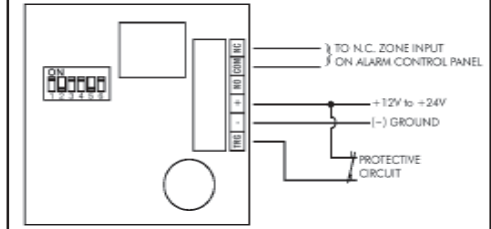
Fig. 3 – Momentary trigger, no delay
