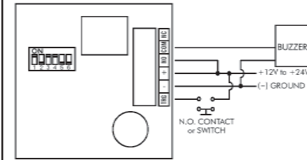
Fig. 2 – Momentary trigger, no delay
