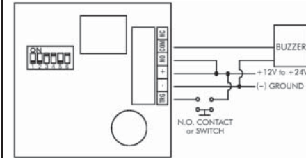
Fig. 4 – 1-time mom. trigger, no delay
