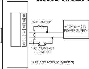
Fig. 7 – Optional negative or closed-circuit trigger
