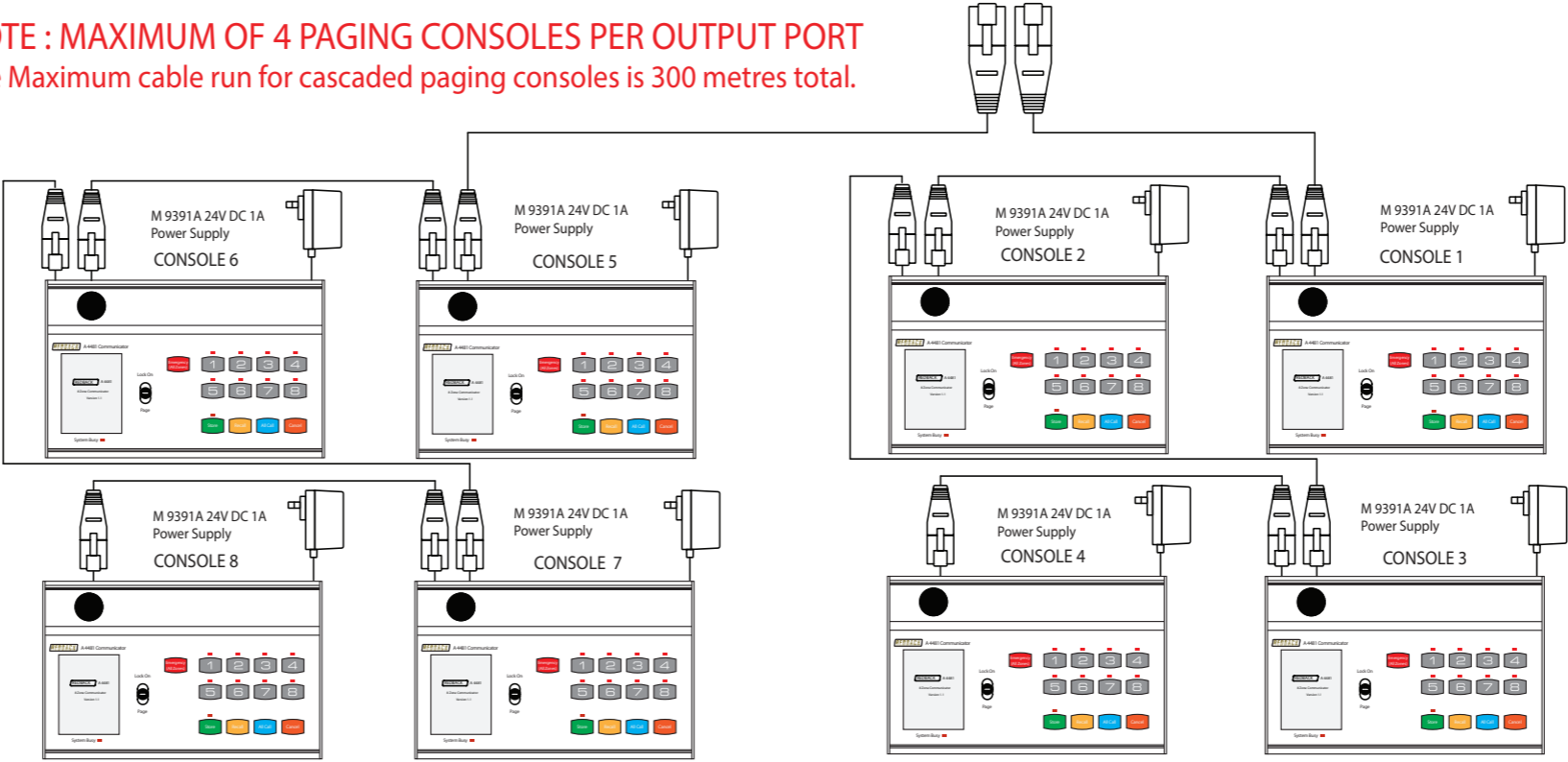
THIS FIGURE ILLUSTRATES HOW TO CONNECT THE MAXIMUM 8 PAGING CONSOLES IN A LOOP IN/LOOP OUT CONFIGURATION ALL WITH SEPARATE EXTERNAL PLUGPACK POWER SUPPLIES (NOT SUPPLIED)
