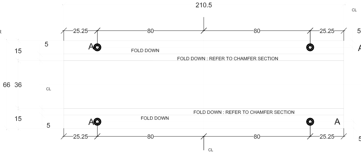
FRONT PANEL PUNCHING DETAILS VIEW FROM FRONT
