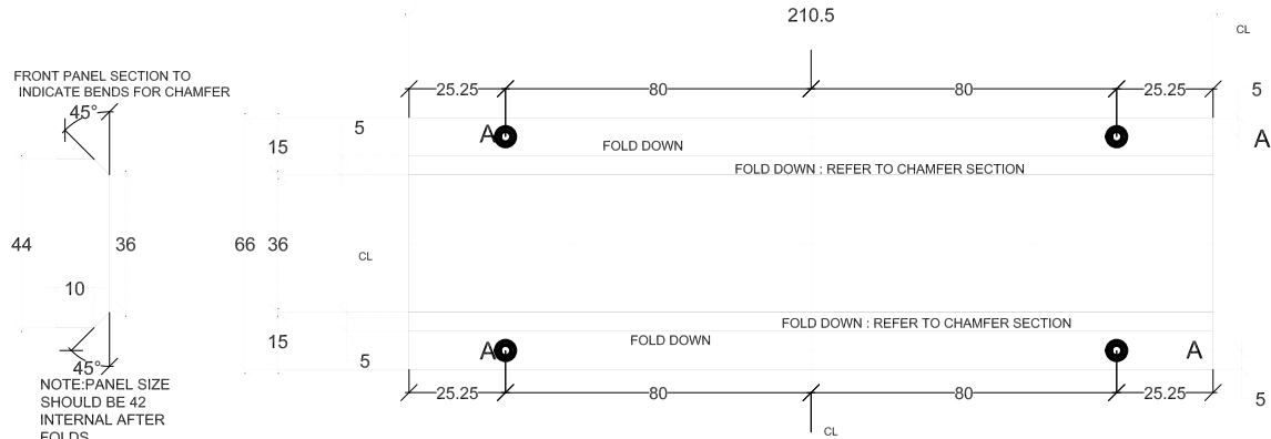
FRONT PANEL PUNCHING DETAILS VIEW FROM FRONT
